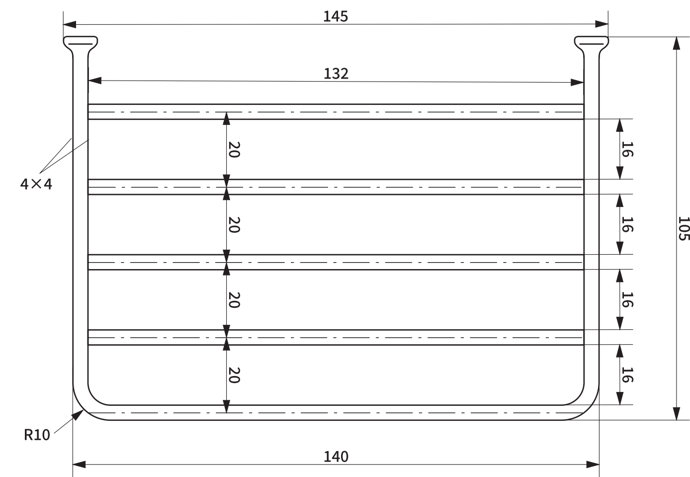
●Front side view (shelf )
