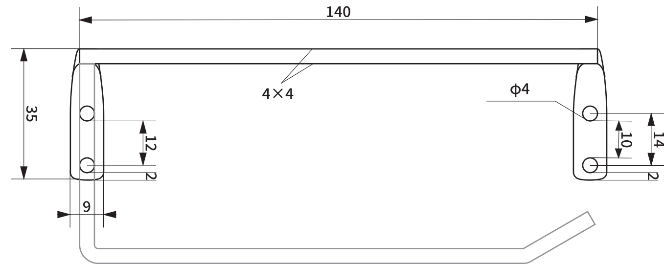
●Front side view (shelf )
