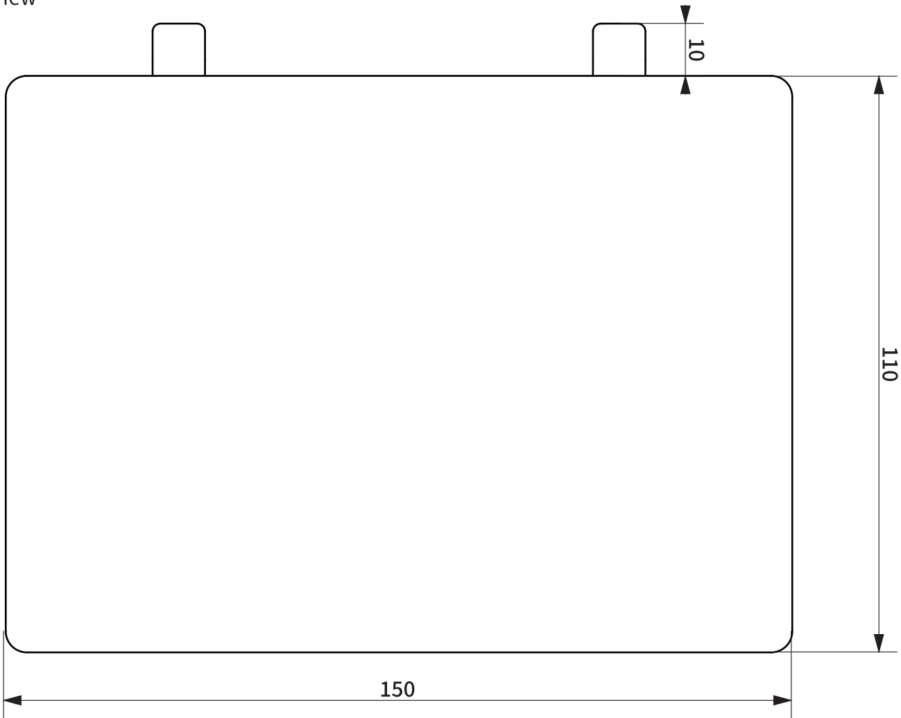
● Top view
