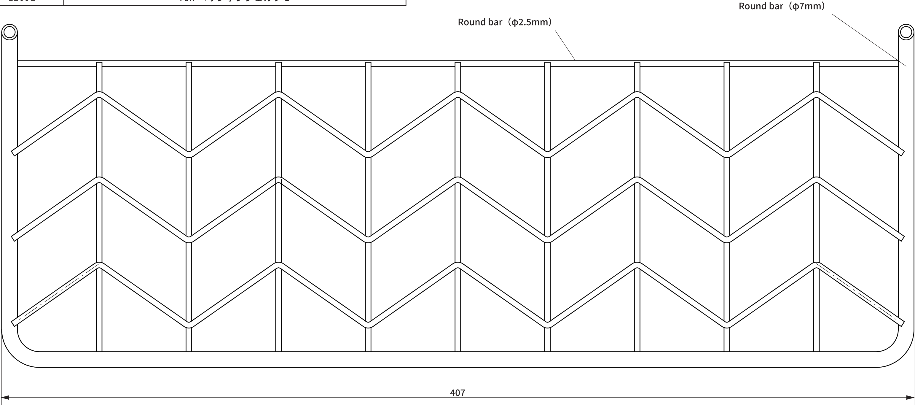
● Top view
