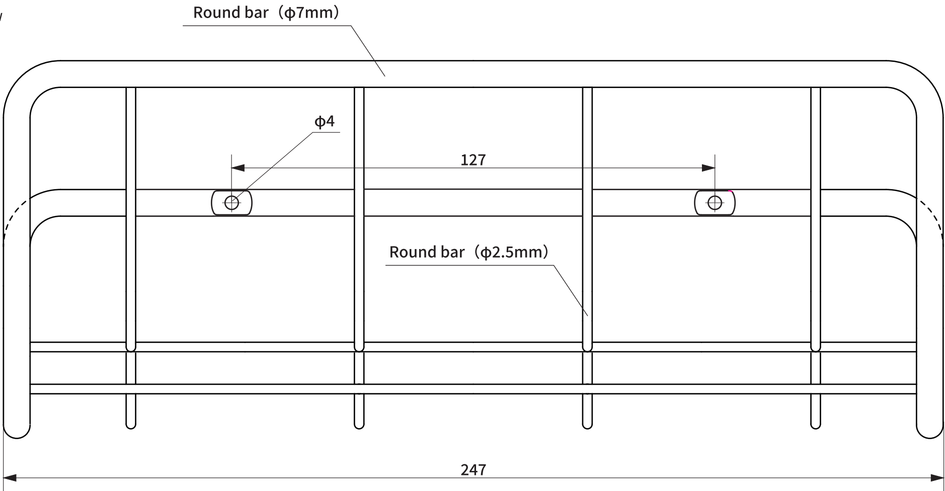
● Front view
