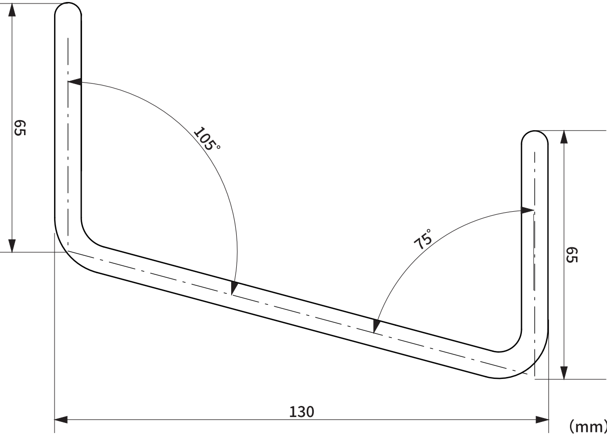
● Side view
