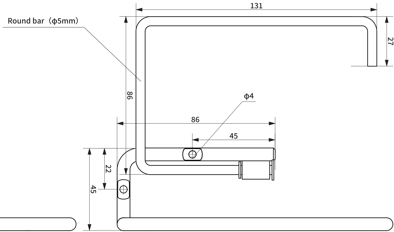
● Front view
