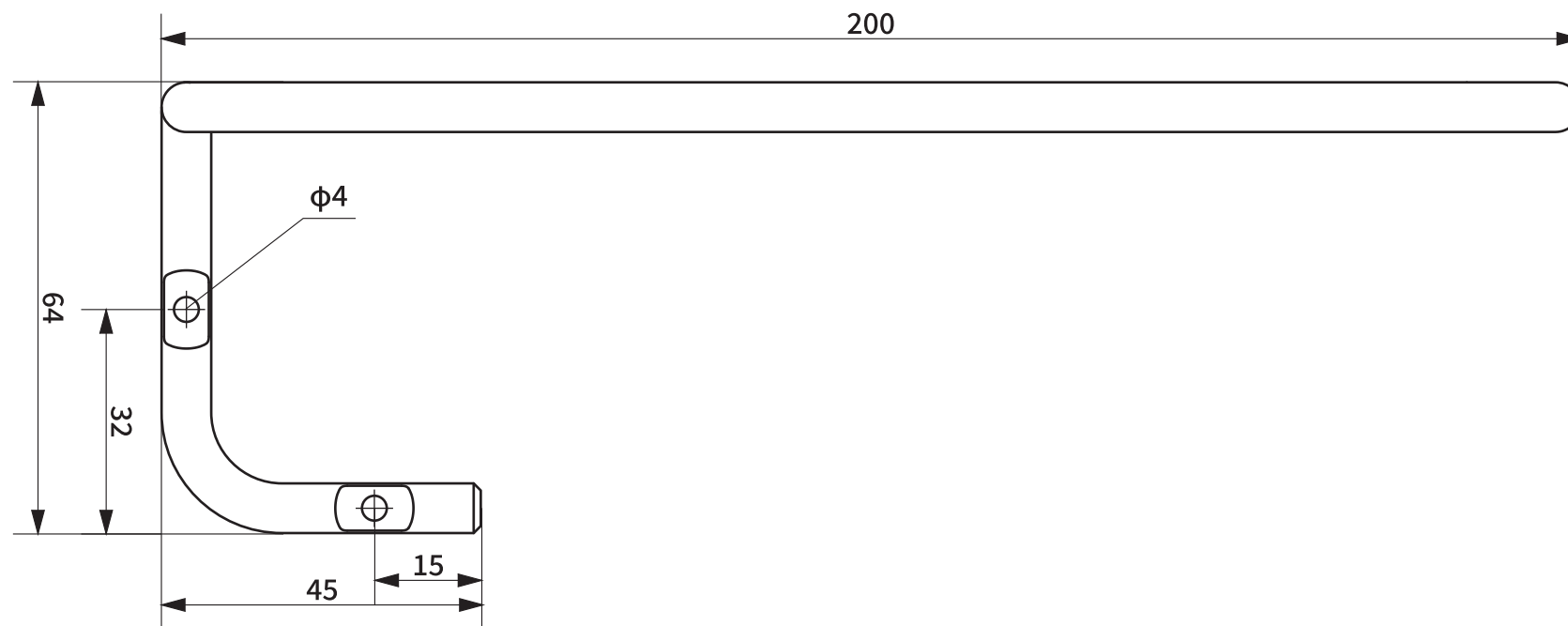
● Front view
