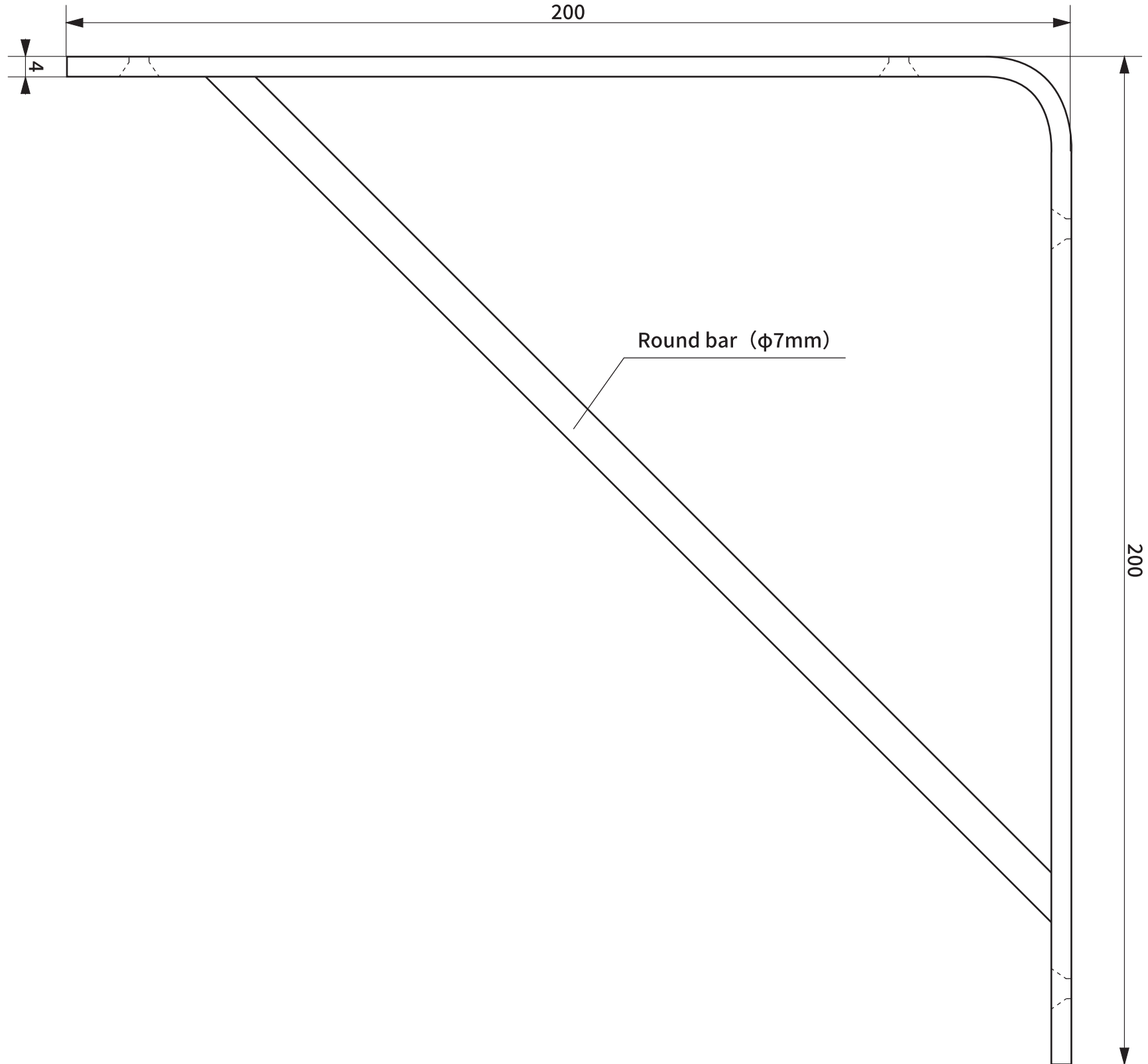
●Side view
