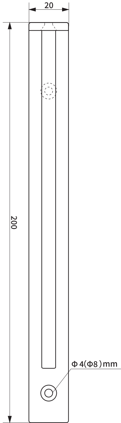
●Front view
